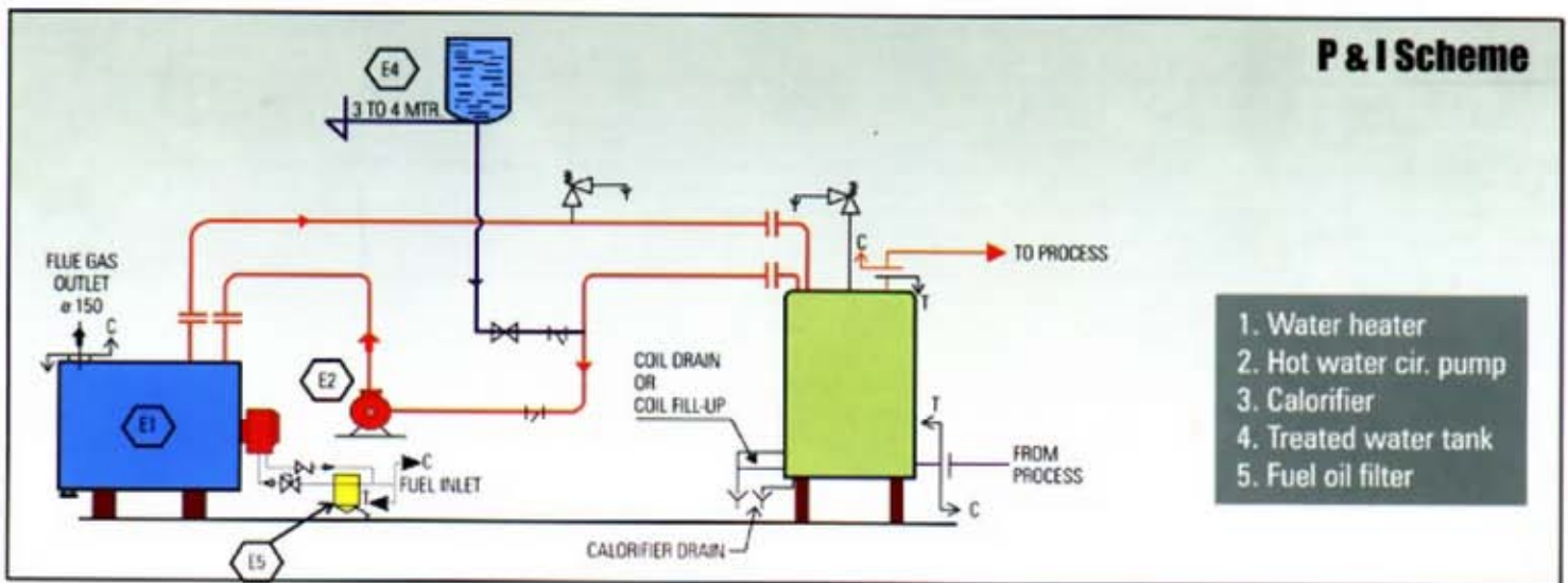
Aquamatic unit with calorifier
