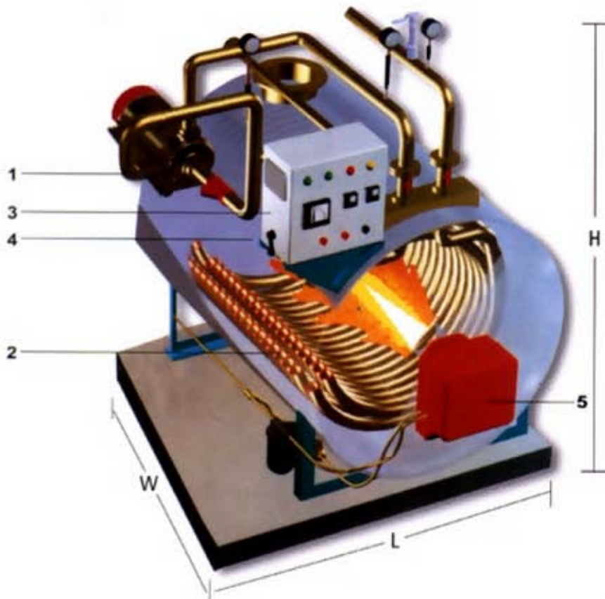
Aquamatic - the inside view
